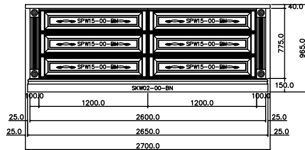
FRONT/BACK VIEW ISLAND - WIC-1A
