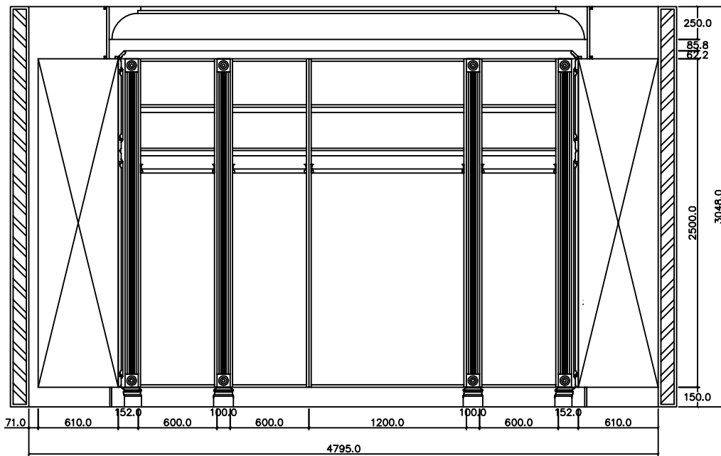
ELEVATION - B W/O DOOR PANEL
