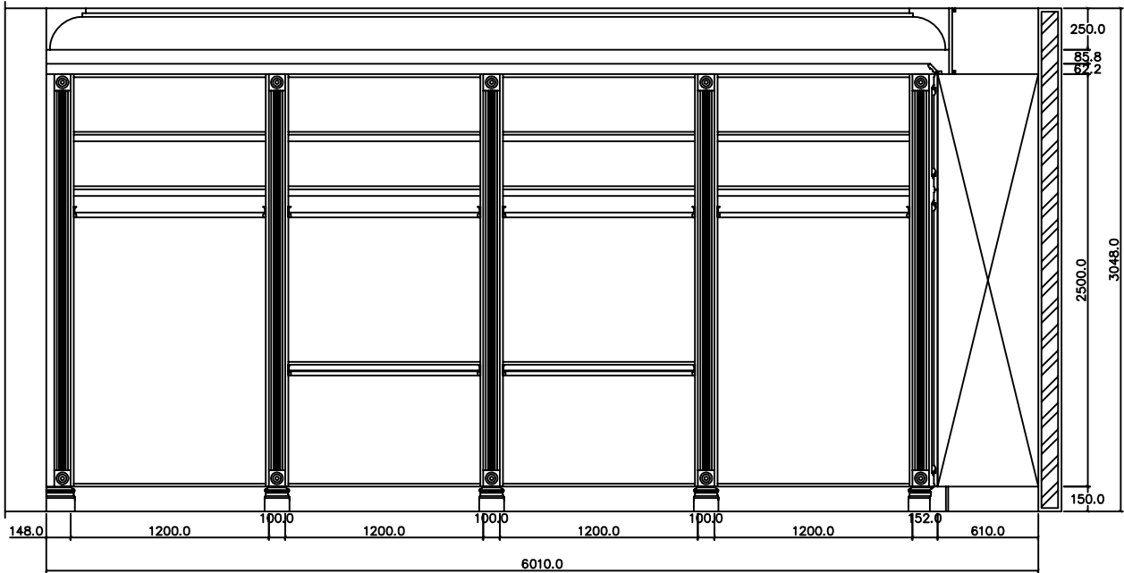
ELEVATION - A W/O DOOR PANEL
