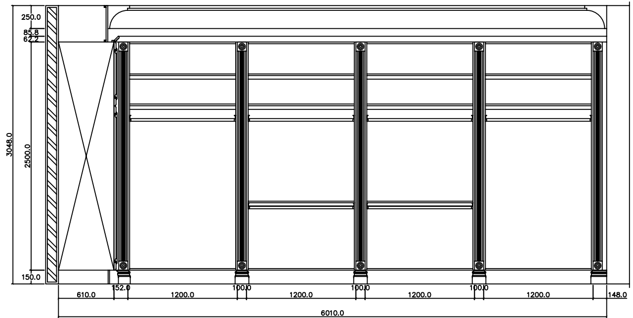
ELEVATION - C W/O DOOR PANEL
