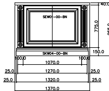
SIDE VIEW ISLAND - WIC-1A
