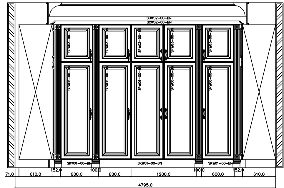
ELEVATION - B WITH DOOR PANEL
