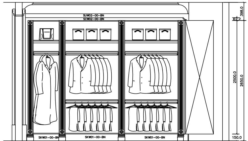
A VIEW
