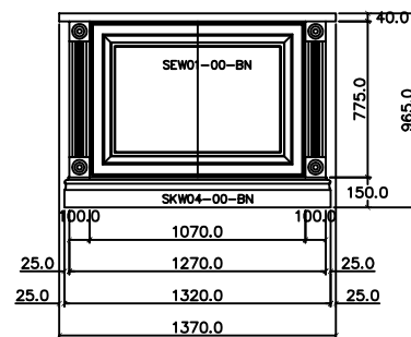
SIDE VIEW ISLAND - WIC-1B
