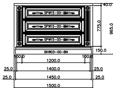
FRONT/BACK VIEW ISLAND - WIC-1B
