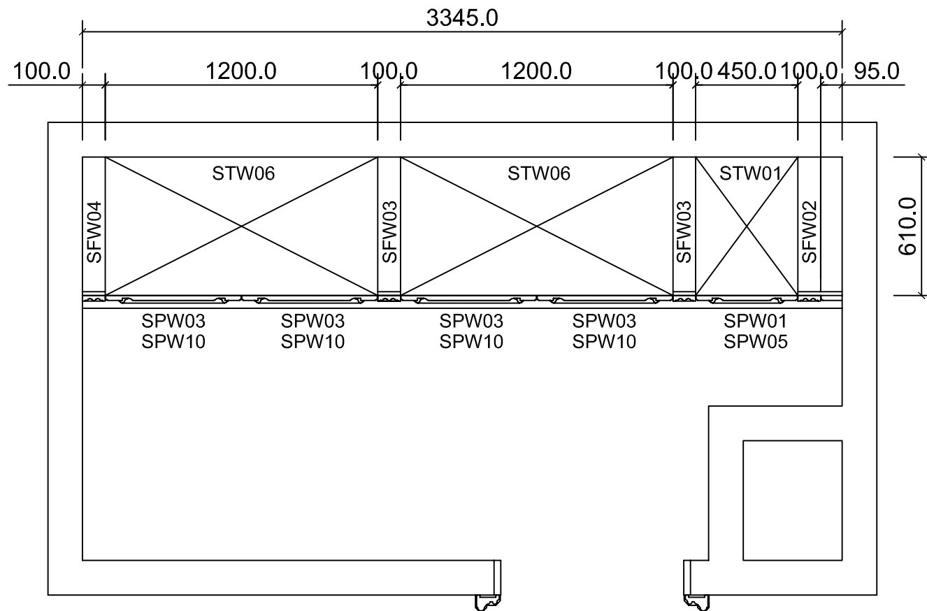
WIC - 6 PLAN
