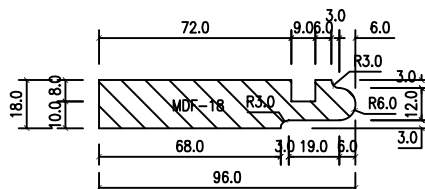
DETAIL 2
