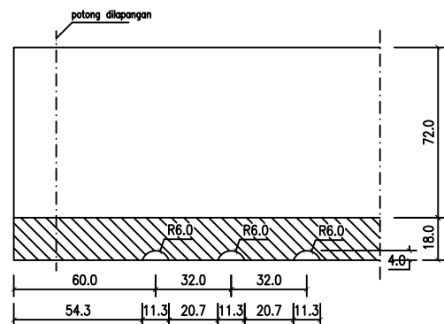
SECTION X-X
