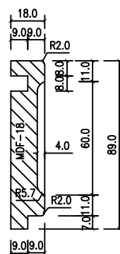
DETAIL 3
