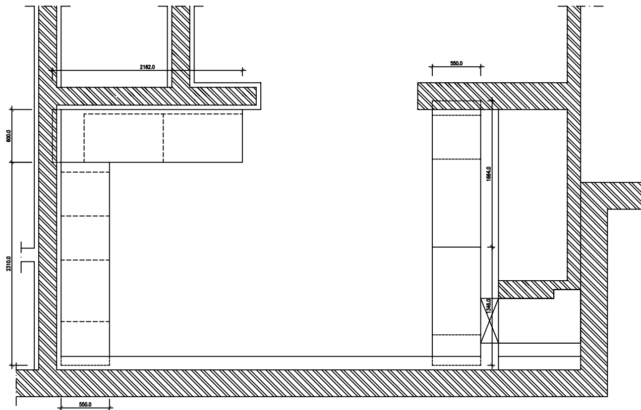
BASE WORKTOP PLAN SNT57-00-WA
