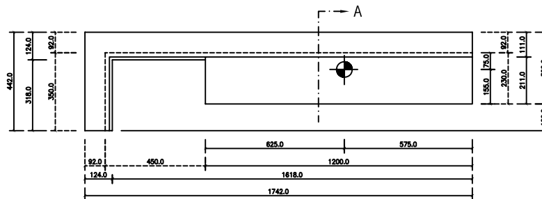
TOP BOARD -3 (SNT63-00-WA)
