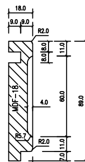
DETAIL 3
