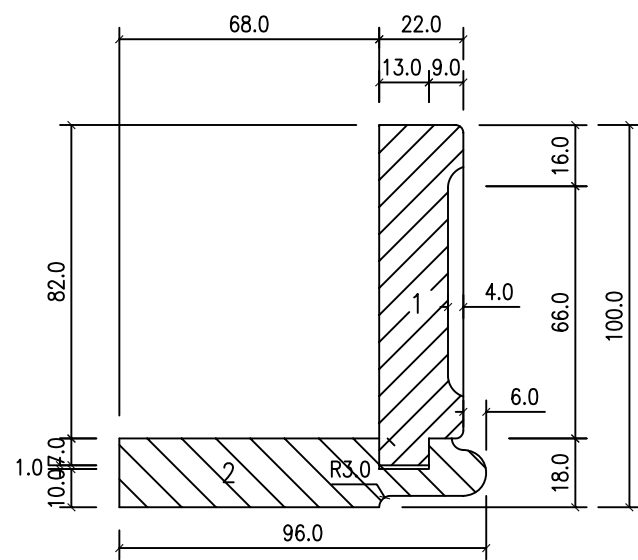
SIDE VIEW DETAIL
