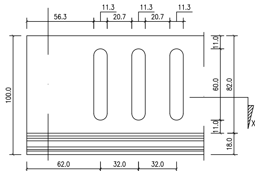
FRONT VIEW DETAIL
