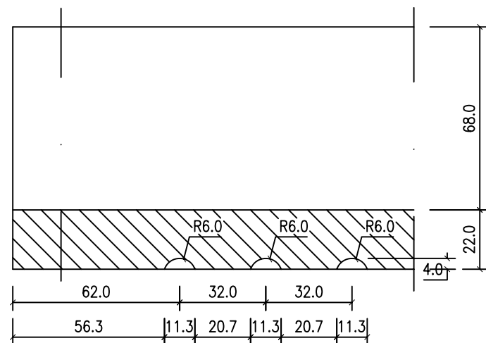
SECTION X-X
