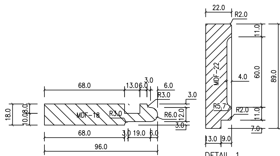
DETAIL 2
