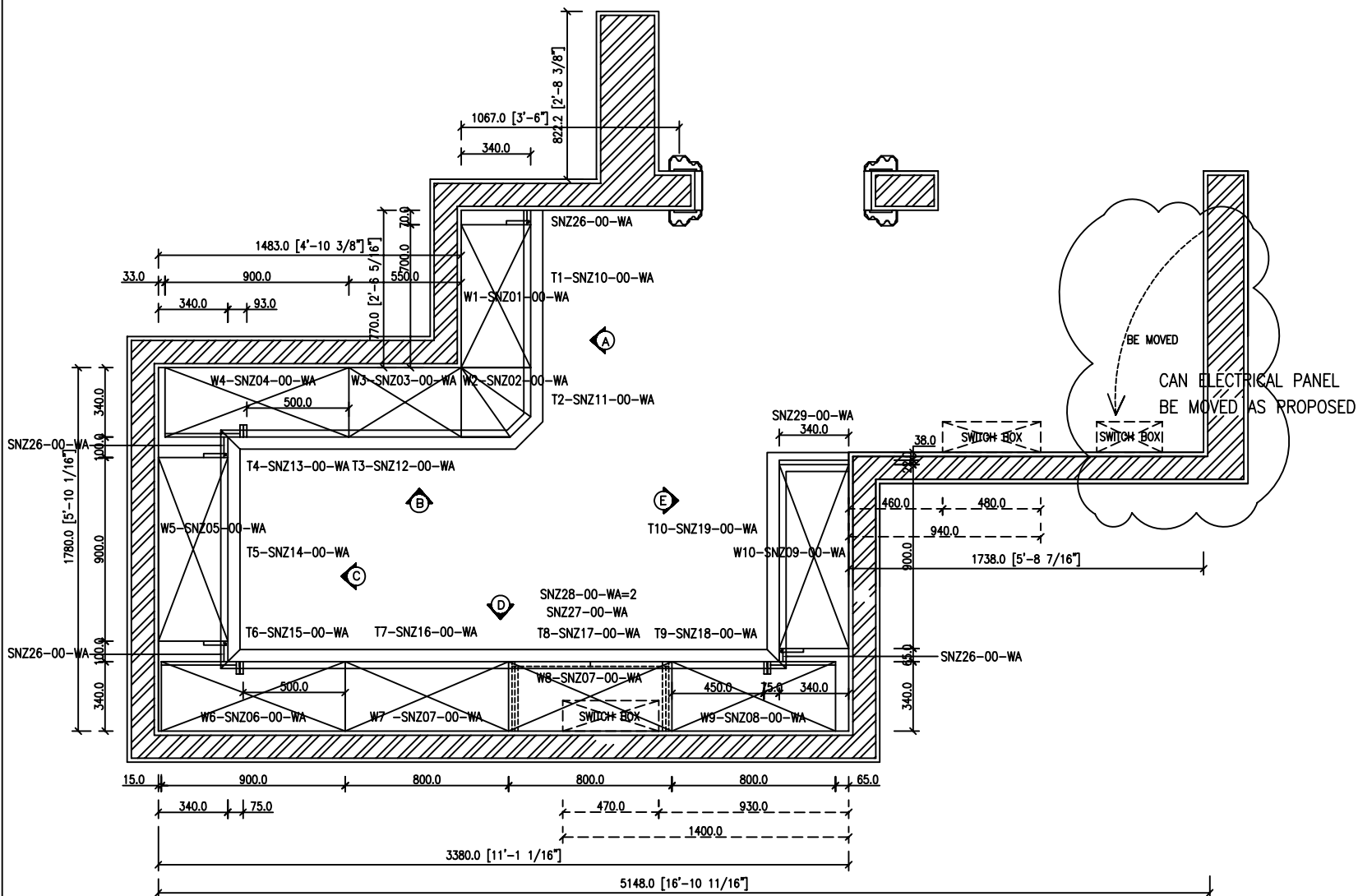
KITCHEN PANTRY LAYOUT PLAN Skala 1 : 20
